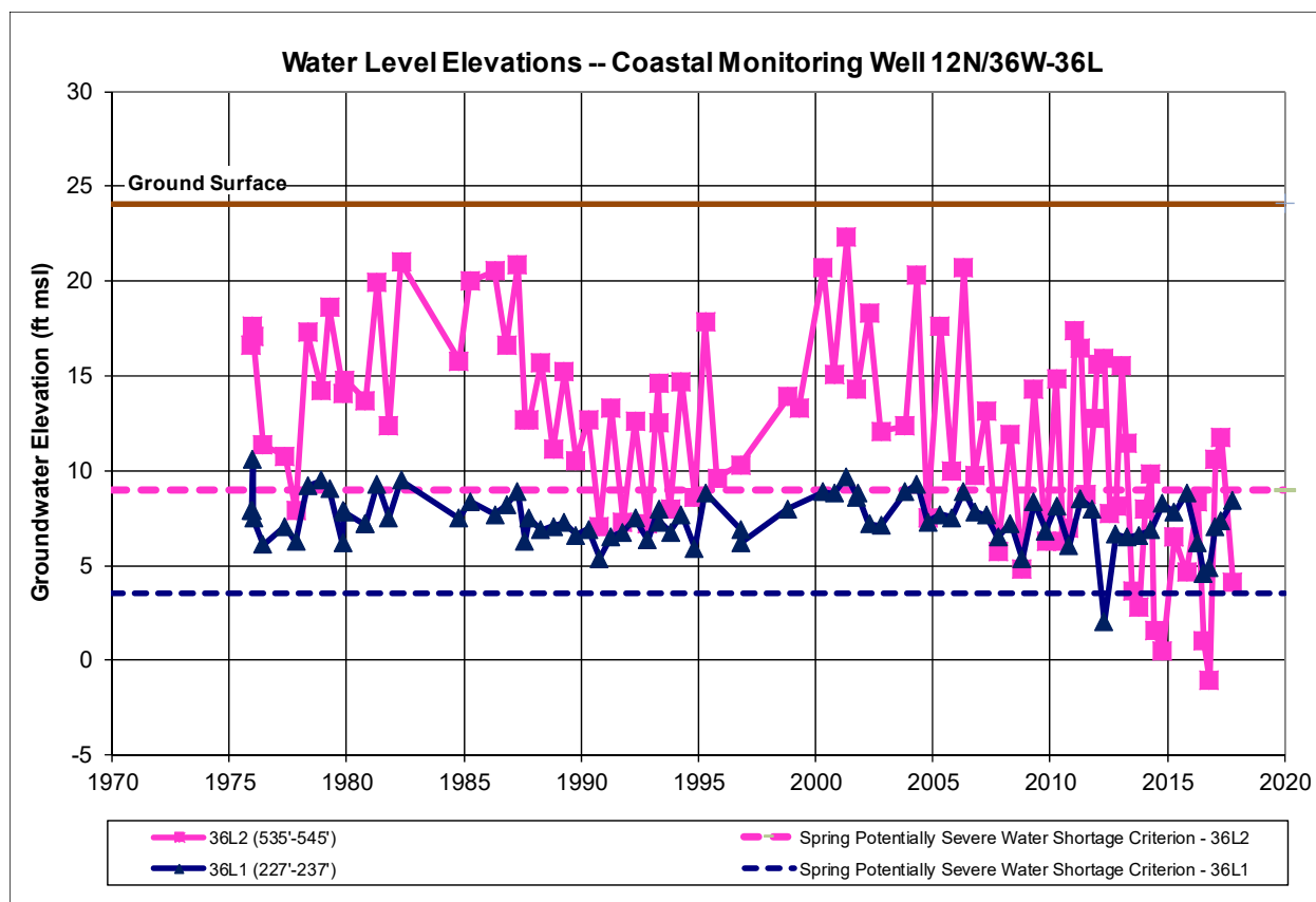
Figure 6-4. Hydrograph for Coastal Monitoring Well Nest 12N/36W-36L
