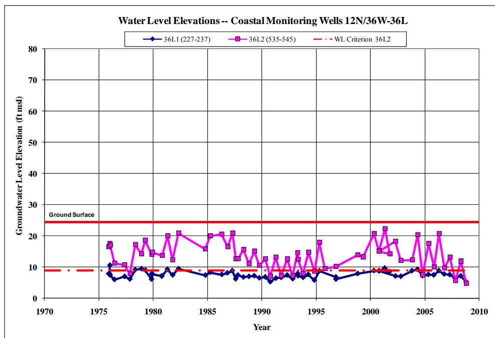
Figure 6-4. Hydrograph for Coastal Monitoring Well Clusters 12N/36W-36L.
