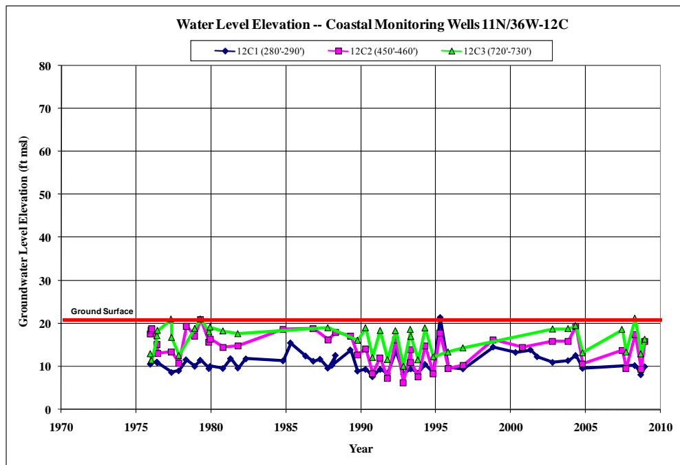
Figure 6-3. Hydrograph for Coastal Monitoring Well Clusters 11N/36W-12C.
